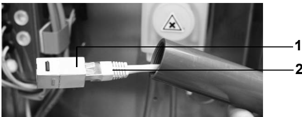
1 Socket
