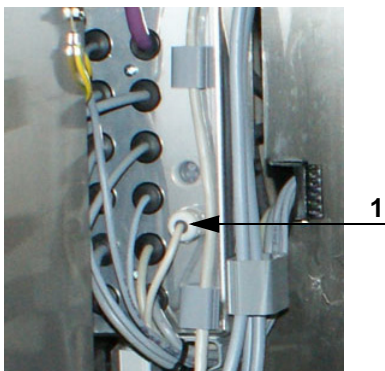
1 Screw fitting for empty signal unit
