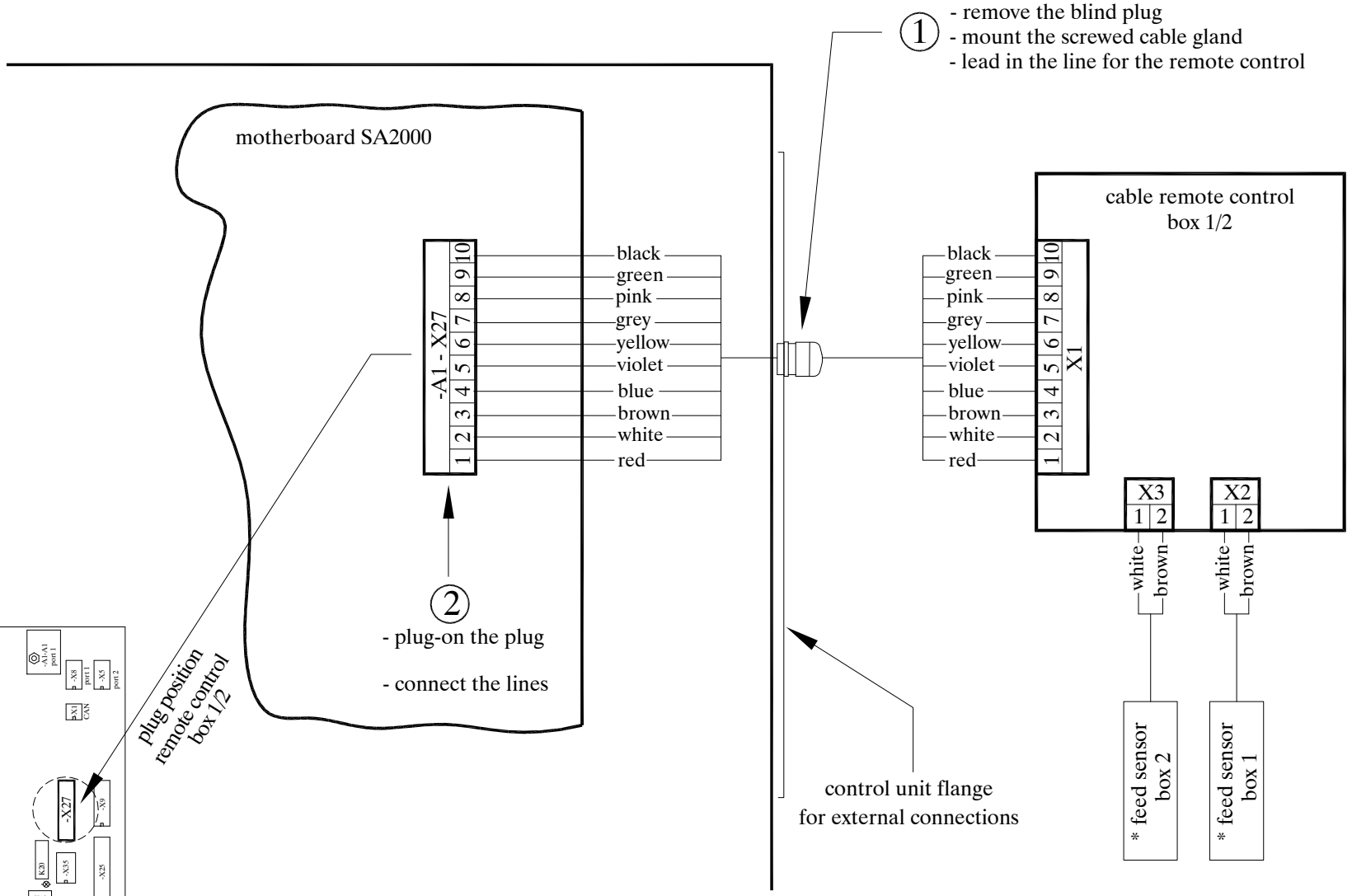
Motherboard
