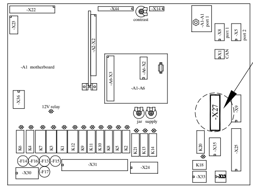
Motherboard
