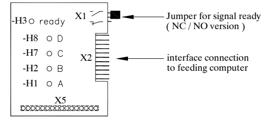
=ST1-A1-A1 relay-interface
