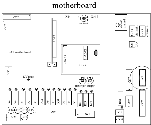
connection identification feeding box 1/2
