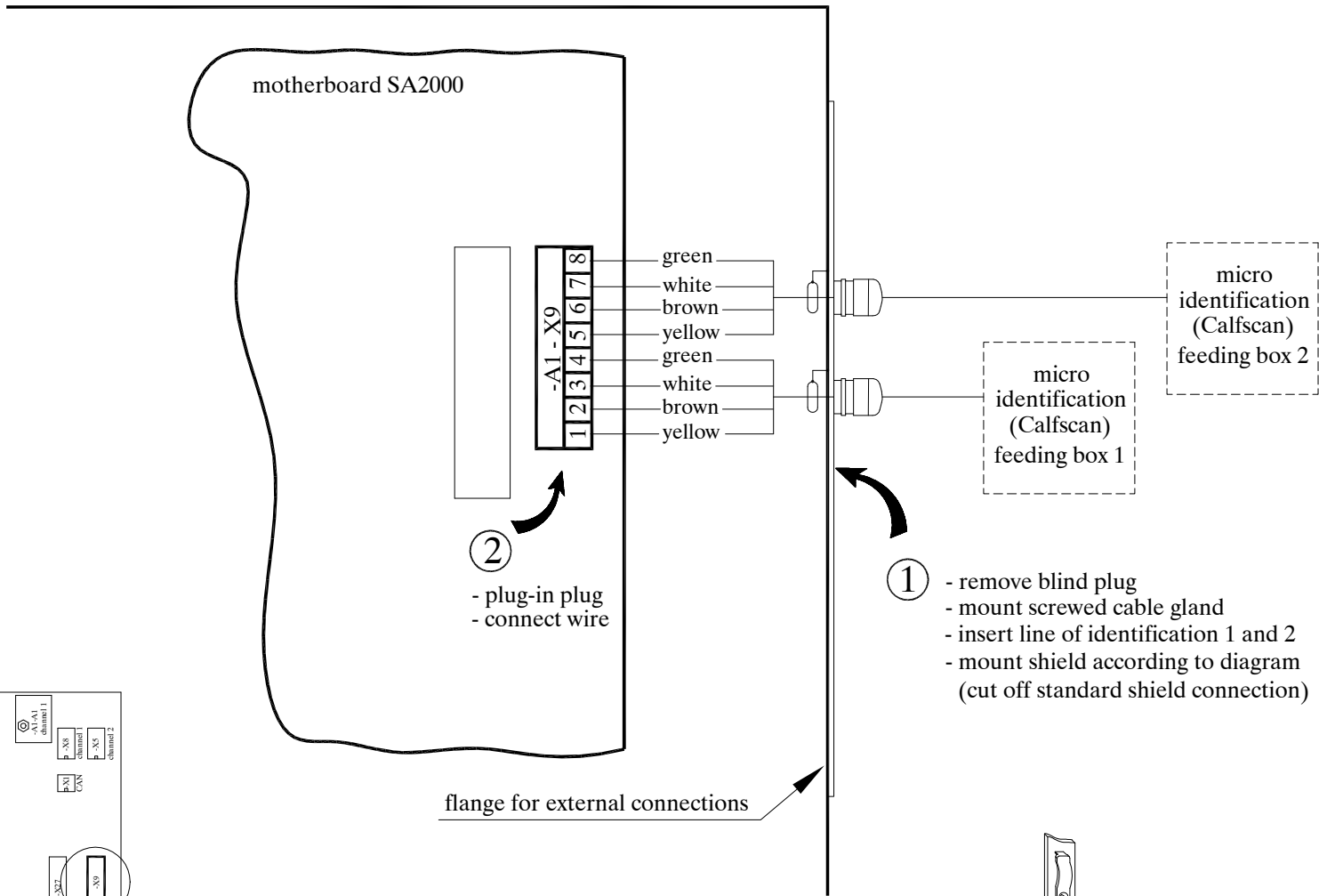
connection identification feeding box 1/2
